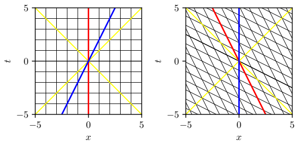
Figure 29: A Lorentz Transformation ( k = 1 )
