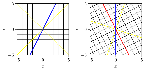
Figure 31: A k < 0 Lorentz Transformation ( k = -1 )
