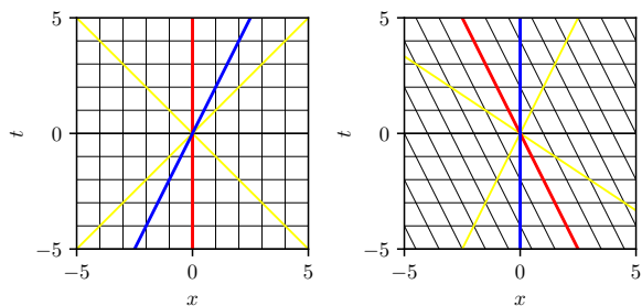
Figure 30: A Galilean Transformation ( k = 0 )
